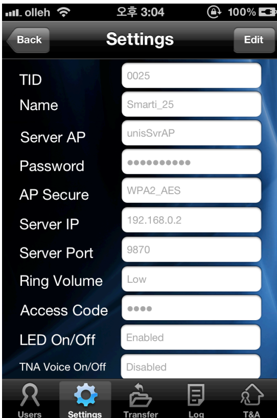
<Terminal Settings Screen>
