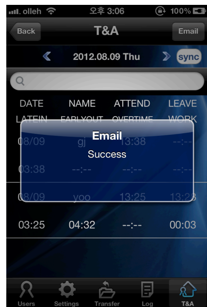
< Email Screen 3 >
