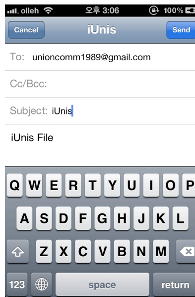
< Email Screen 2 >
